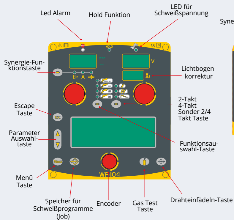
Frontbedienfeld WF104
