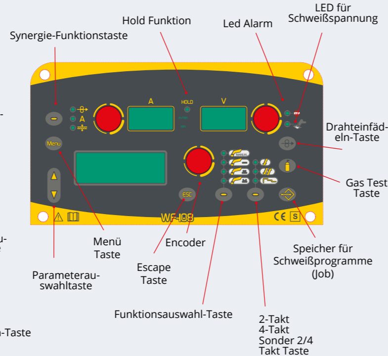
Frontbedienfeld WF108
